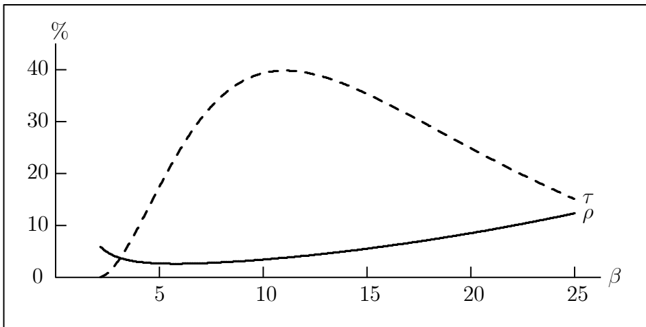
Figure 9: Probability of reversion \rho and of investigation \tau as functions of \beta . a = 110 , c = 10 , b = 1 , r = 1/10 , U = 50 , \omega = 1/5 , F = 625 .
