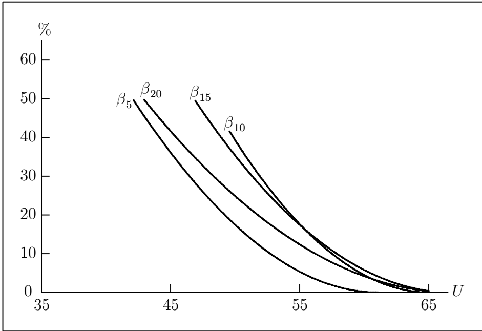
Figure 8: Probability of investigation \tau as a function of investigation threshold U . a = 110 , c = 10 , b = 1 , r = 1/10 , \beta = 5, 10, 15, 20 , n = 2 , \omega = 1/5 , F = 625 .
