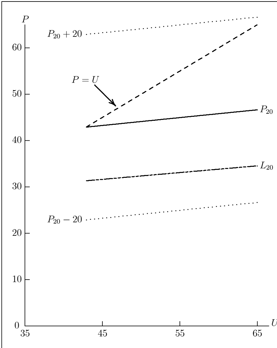
Figure 6: Tacit collusion price P , and reversion threshold L as function of investigation threshold U . a = 110 , c = 10 , b = 1 , r = 1/10 , \beta = 20 , n = 2 , \omega = 1/5 , F = 625 .
