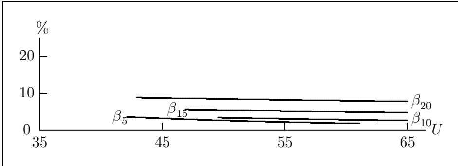
Figure 7: Probability of reversion \rho as a function of investigation threshold U . a = 110 , c = 10 , b = 1 , r = 1/10 , n = 2 , \omega = 1/5 , F = 625 .
