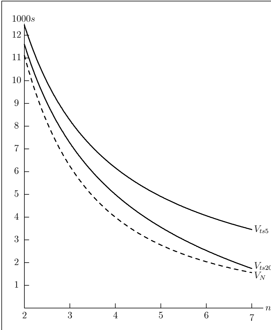
Figure 4: One-shot game and trigger-strategy equilibrium firm value as functions of number of firms; a = 110 , c = 10 , b = 1 , r = 1/10 , \beta = 5 and \beta = 20 .
