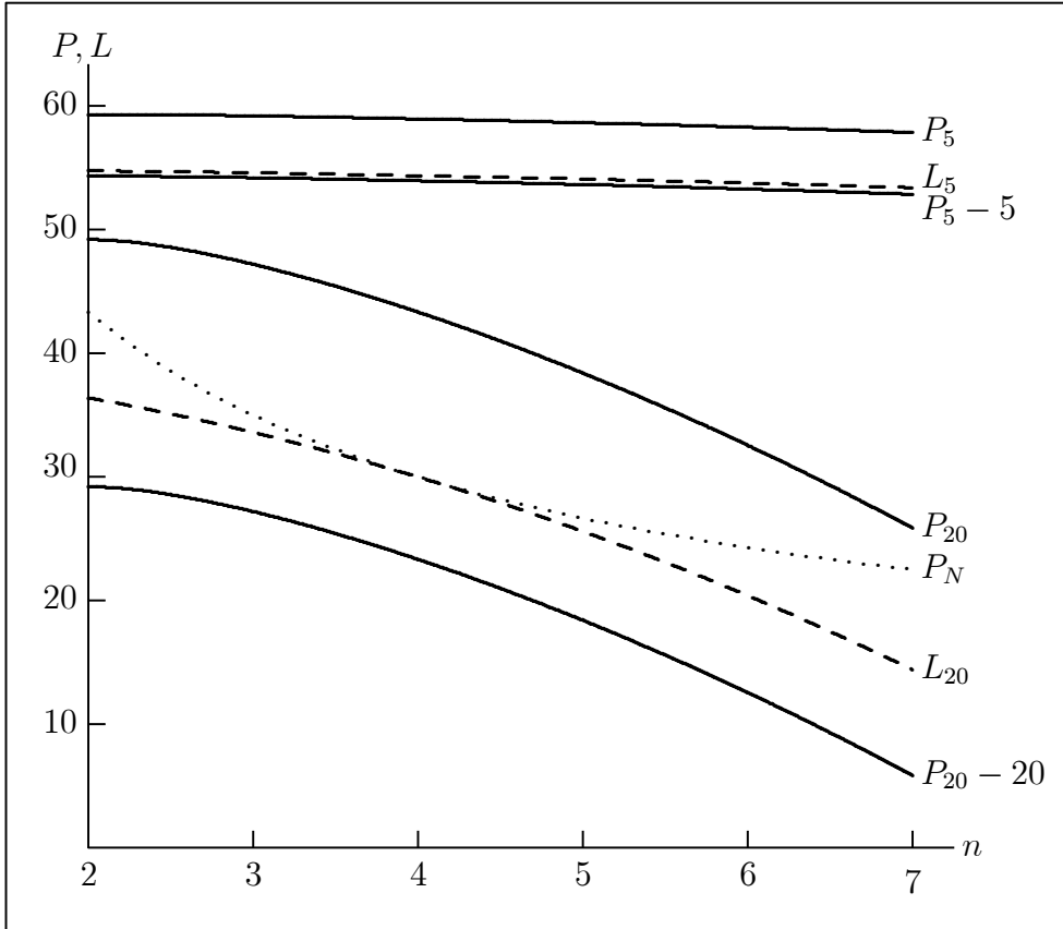
Figure 3: Trigger strategy price P , reversion threshold L , P - \beta , and one-shot game Nash-Cournot price P_N , as functions of number of firms; a = 110 , c = 10 , b = 1 , r = 1/10 , \beta = 5 and \beta = 20 .
